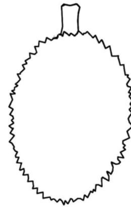
3 elliptic
